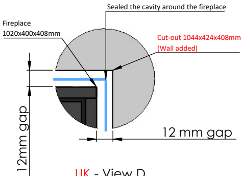
UK - View D 1:2
